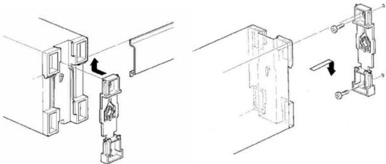
Rail mounting
